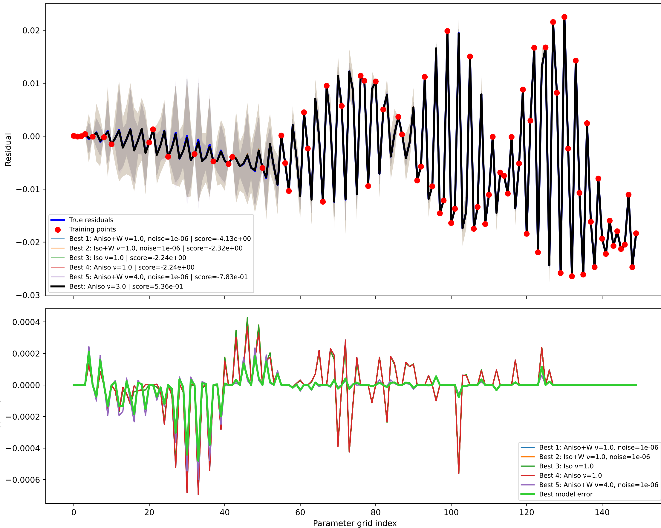
GPR kernel comparison node=22 RMSE=8.315e-05, train RMSE=1.805e-11
